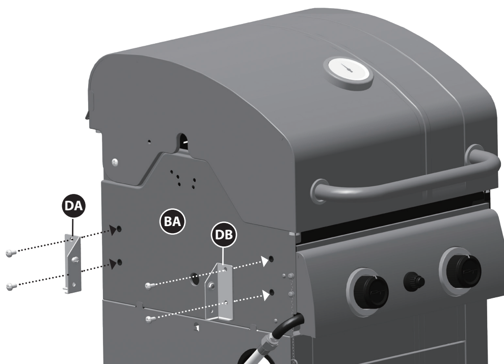
SUPPORT BRACKET A (DA)
